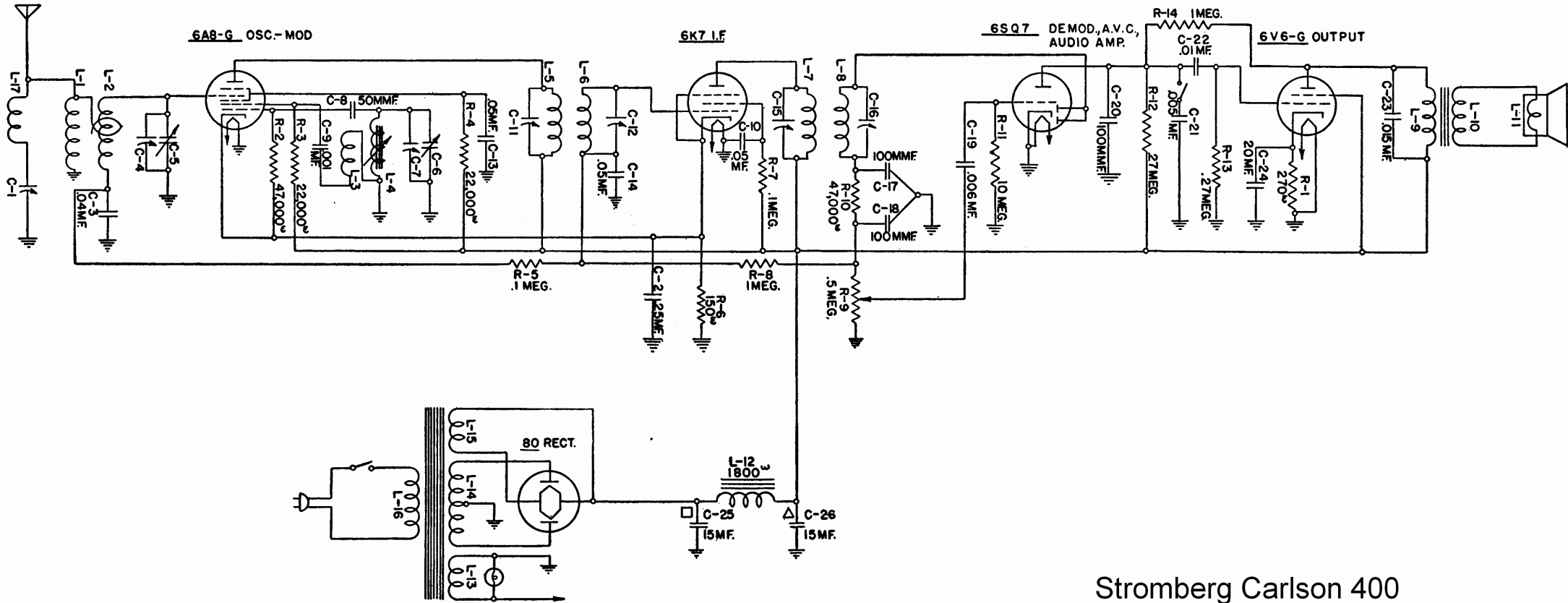
Schematic Circuit
